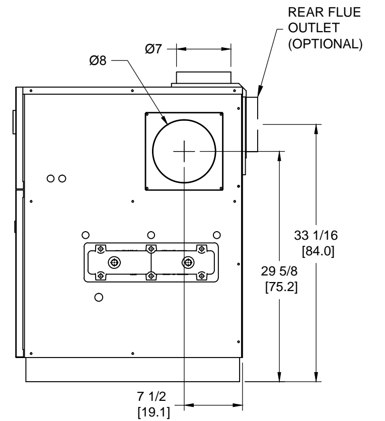
RIGHT VIEW
